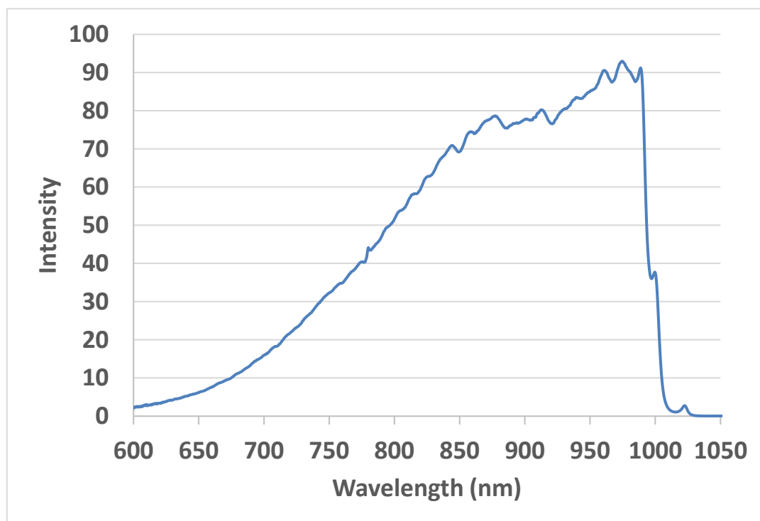
SC-OCT Typical Spectrum
